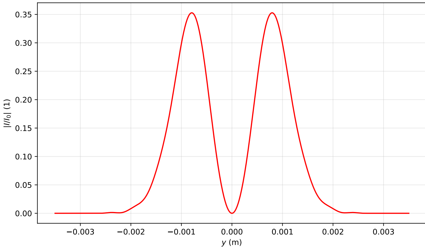
Intensity profile I(x=0, y, z=2.866)/I_0 , \text{Pin}=2.0\text{Pcr} , artificial time
